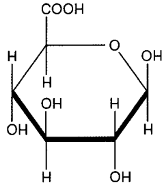
Figure 1. Structural formula of glucuronic acid (M.W. 194.1).
